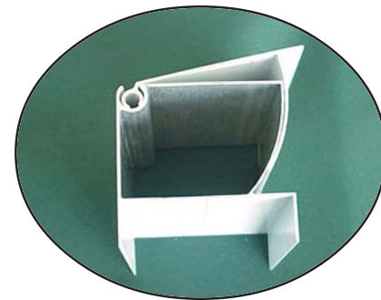
ADJUSTABLE HEADER Designed to match site lines and evenly distribute the weight on the load bearing wall.
