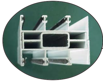
MULLION / SIDE JAMBS Connected with a hidden extruded aluminum mullion to prevent racking and flexing of the frame. Hidden connections inside the side jambs offer a more pleasing look.
