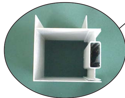
CORNER POST Extruded aluminum to prevent racking and twisting of the wall system, reinforced with the hidden mullion.
