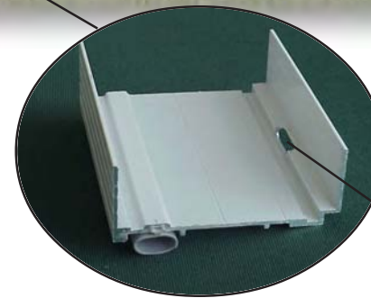
FLOOR CHANNEL SYSTEM Built-in pitch, channels for the sill gasket and pre-punched, elongated hidden weep holes all work to direct water away from the patio room. Installation techniques insure proper caulking and lag placement to meet or exceed building codes.
